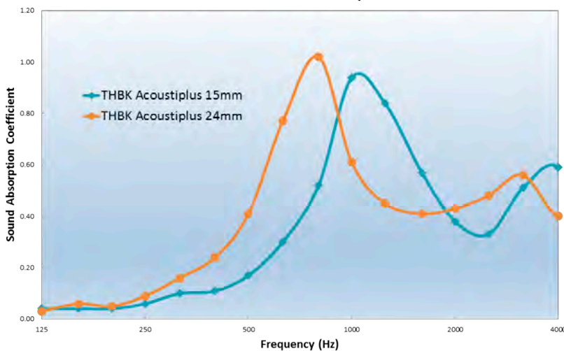
Thermobreak ® AcoustiPlus Sound Absorption Coefficients
